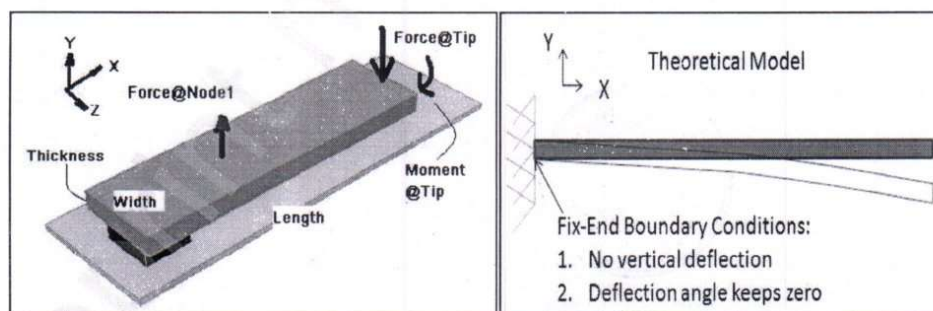
Fig. 5 - Experimental Modal.
